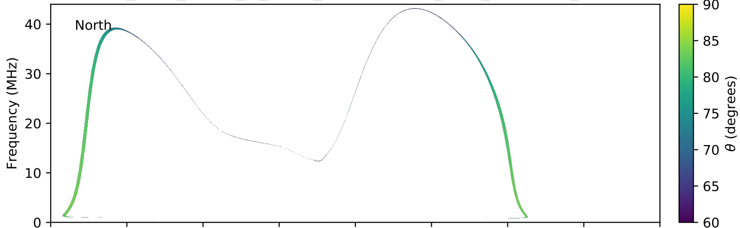
expres_earth_jupiter_io_jrm09_lossc-wid1deg_3kev_20041111_v11.cdf
