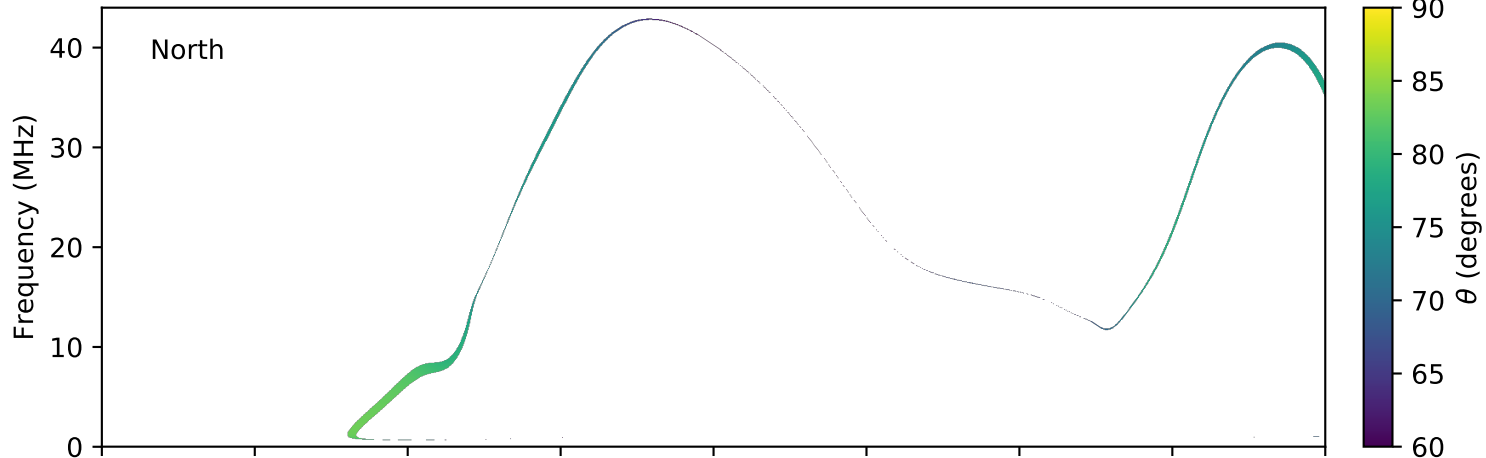
expres_earth_jupiter_io_jrm09_lossc-wid1deg_3kev_20041109_v11.cdf
