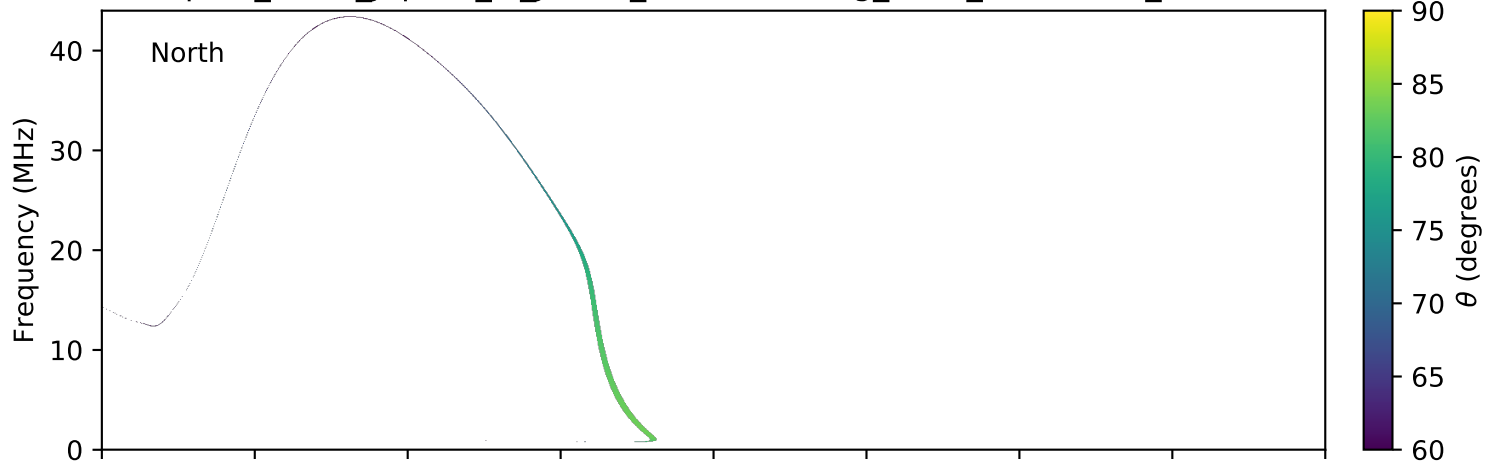
expres_earth_jupiter_io_jrm09_lossc-wid1deg_3kev_20041106_v11.cdf
