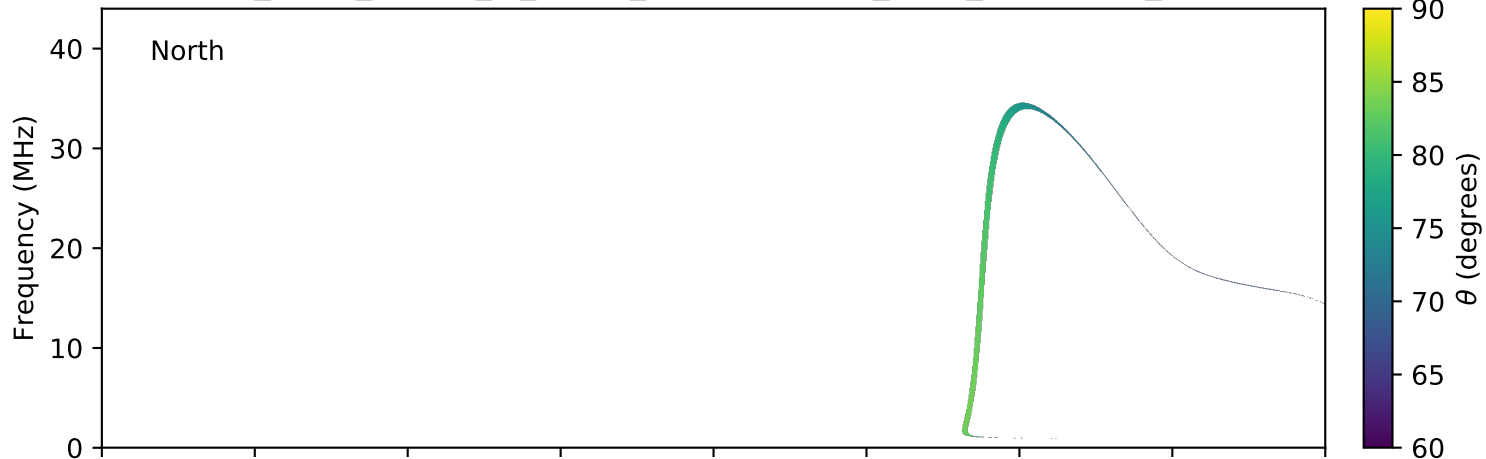
expres_earth_jupiter_io_jrm09_lossc-wid1deg_3kev_20041105_v11.cdf
