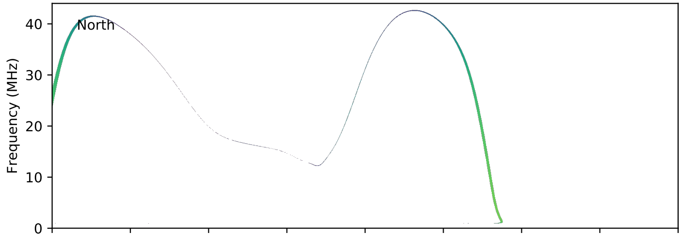
expres_earth_jupiter_io_jrm09_lossc-wid1deg_3kev_20041104_v11.cdf
