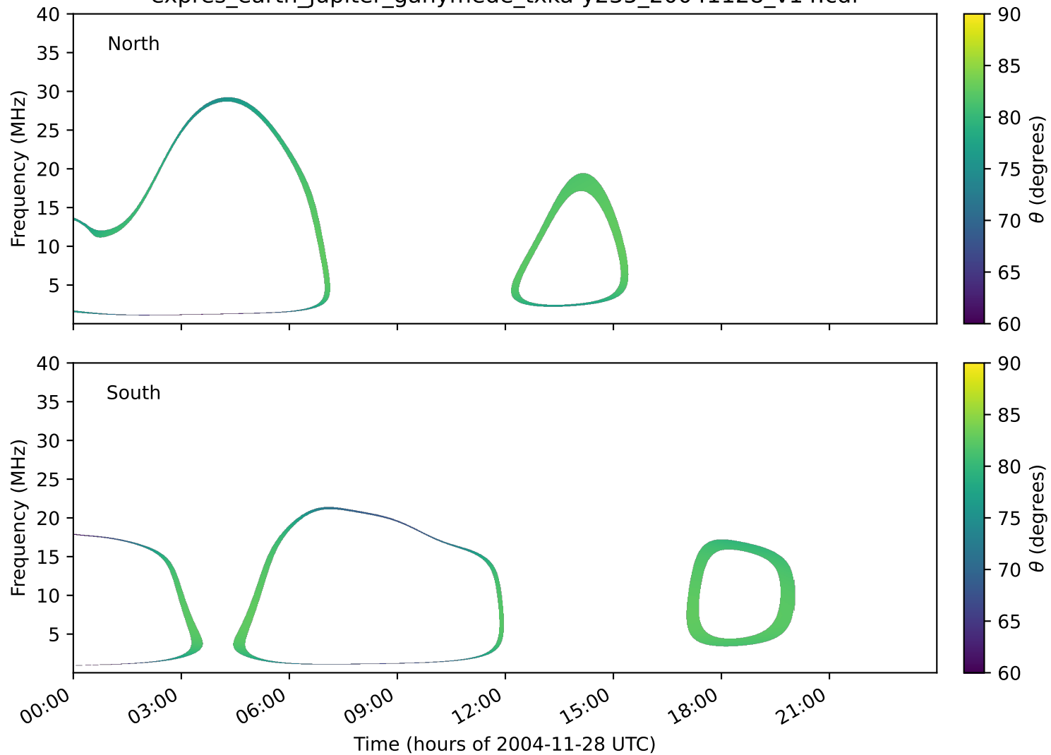
expres_earth_jupiter_ganymede_txka-y235_20041128_v14.cdf
