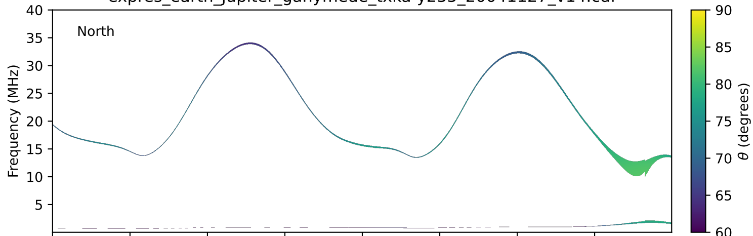
expres_earth_jupiter_ganymede_txka-y235_20041127_v14.cdf
