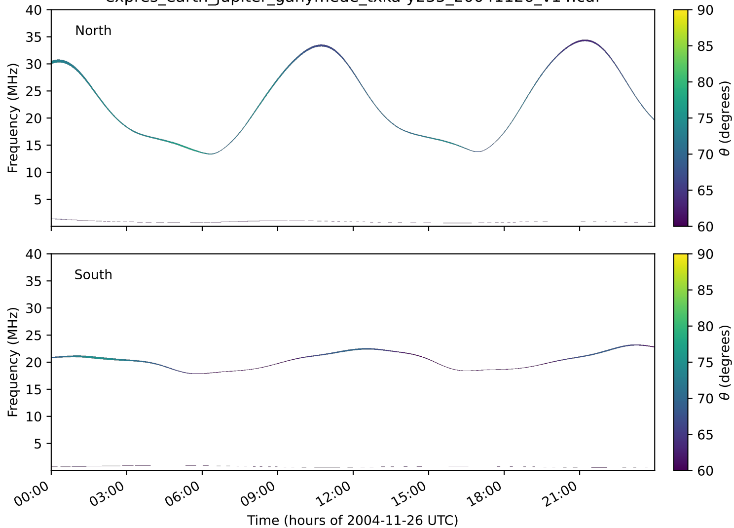
expres_earth_jupiter_ganymede_txka-y235_20041126_v14.cdf
