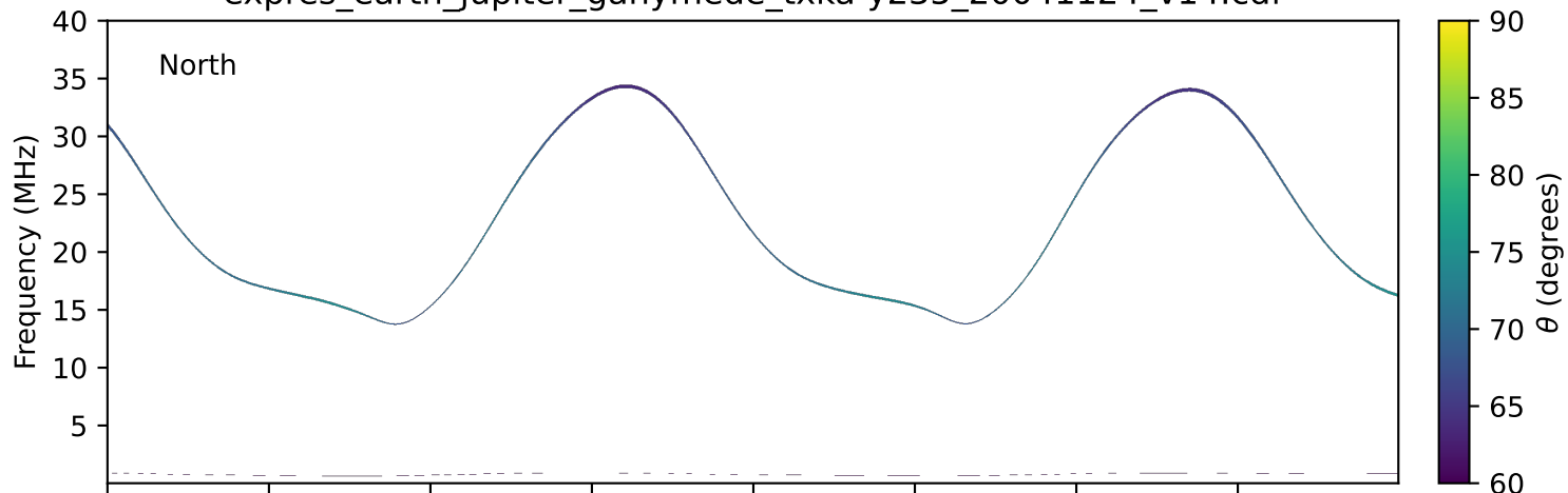
expres_earth_jupiter_ganymede_txka-y235_20041124_v14.cdf
