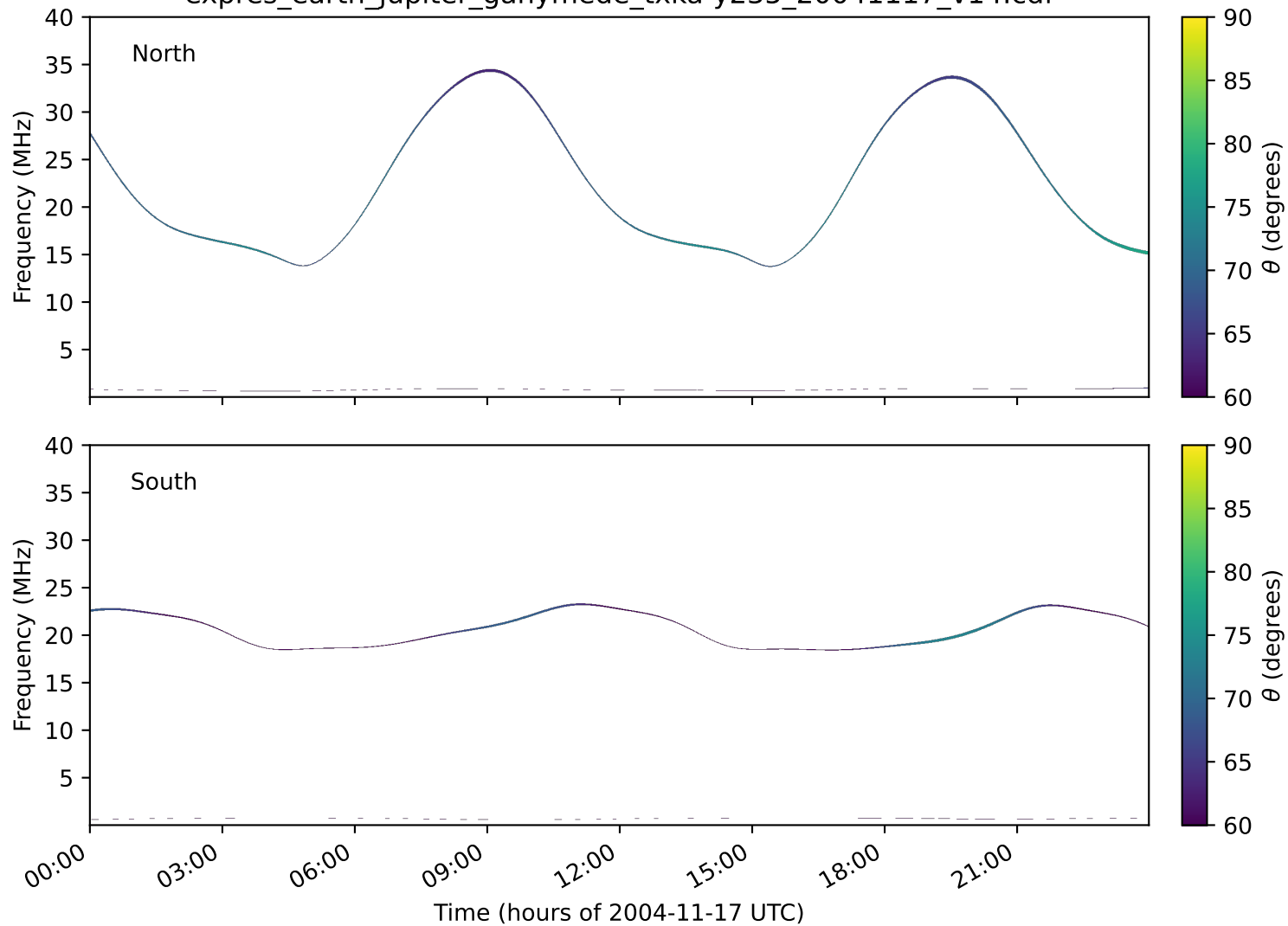
expres_earth_jupiter_ganymede_txka-y235_20041117_v14.cdf
