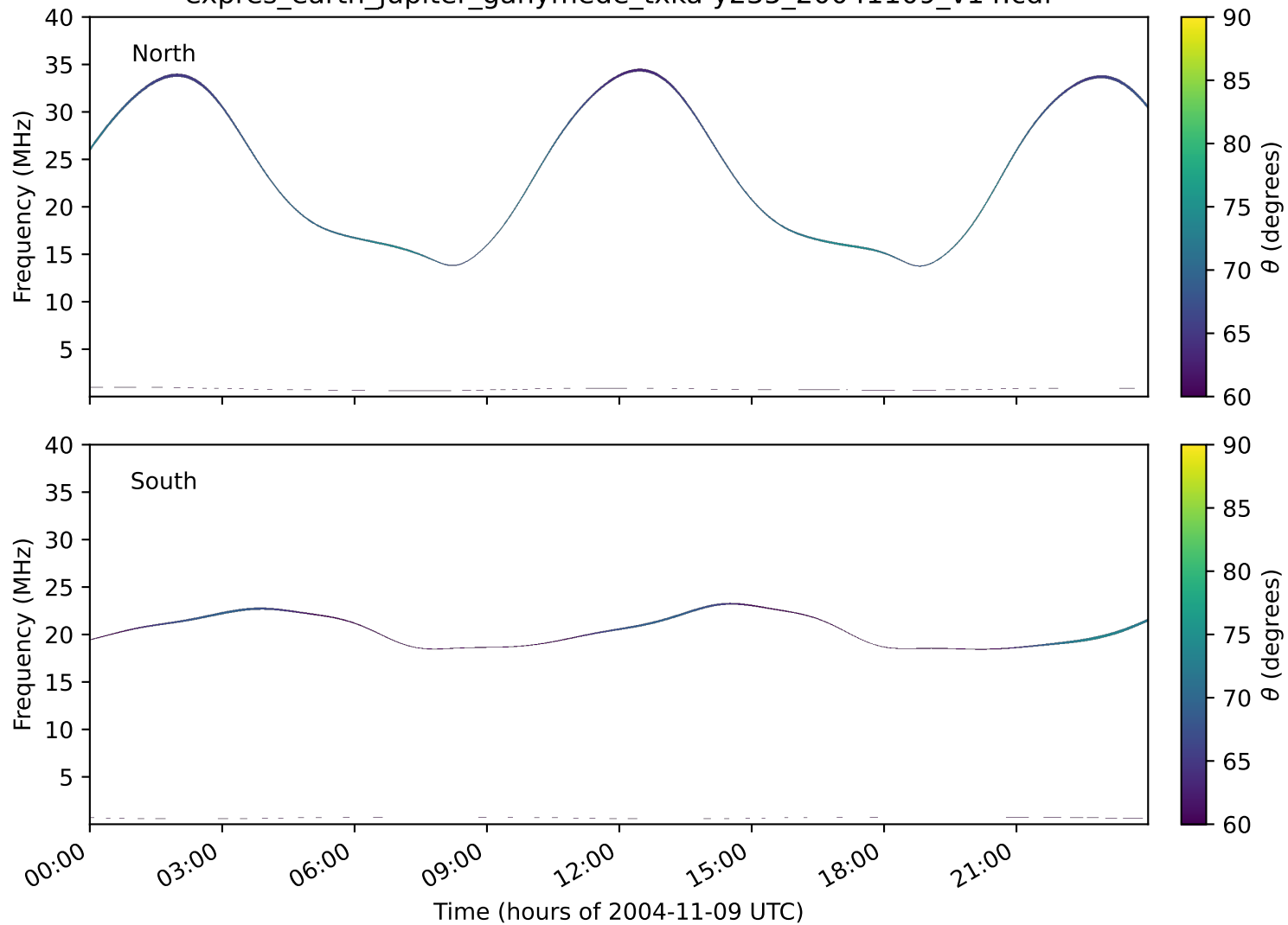
expres_earth_jupiter_ganymede_txka-y235_20041109_v14.cdf
