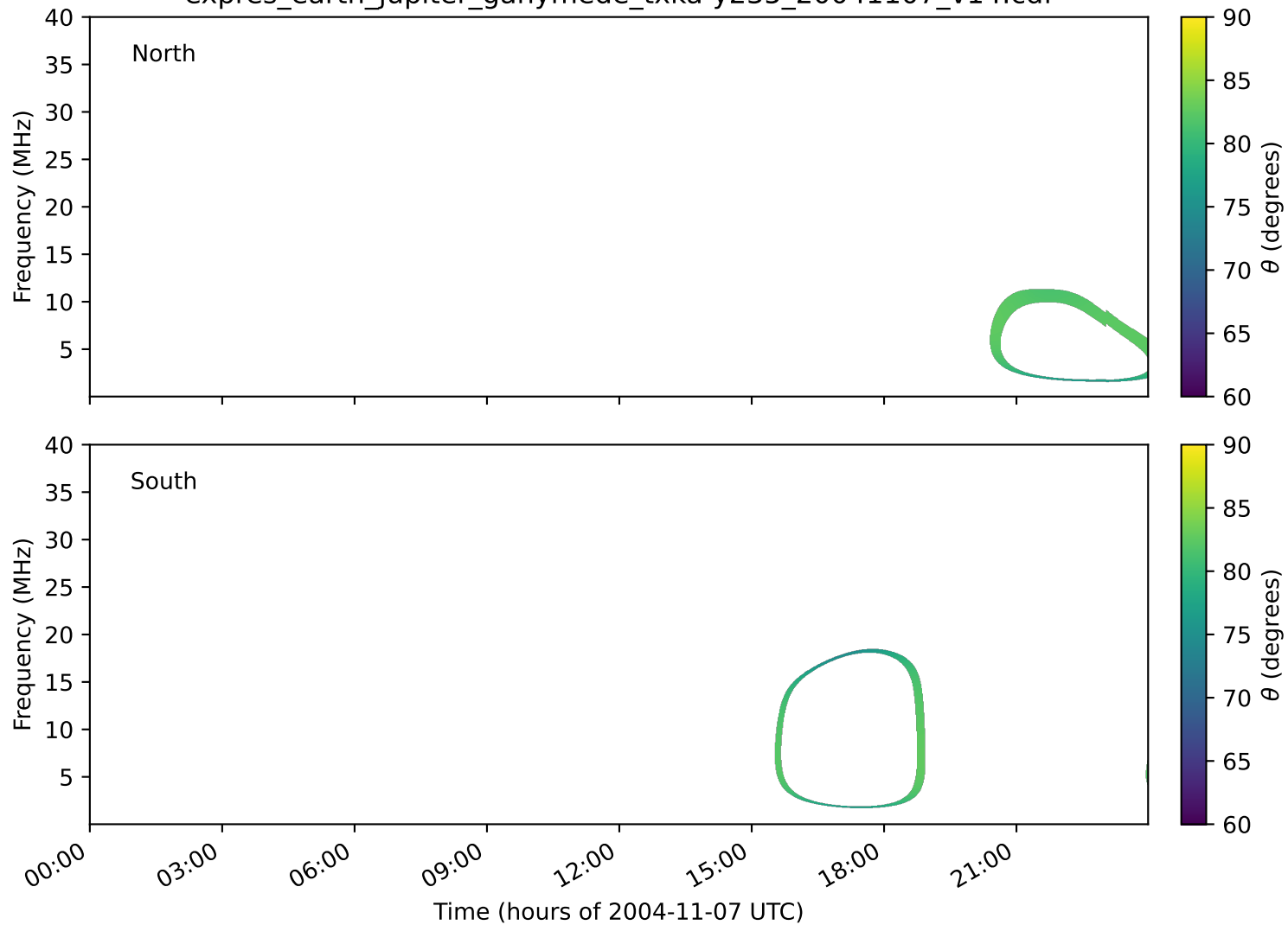
expres_earth_jupiter_ganymede_txka-y235_20041107_v14.cdf
