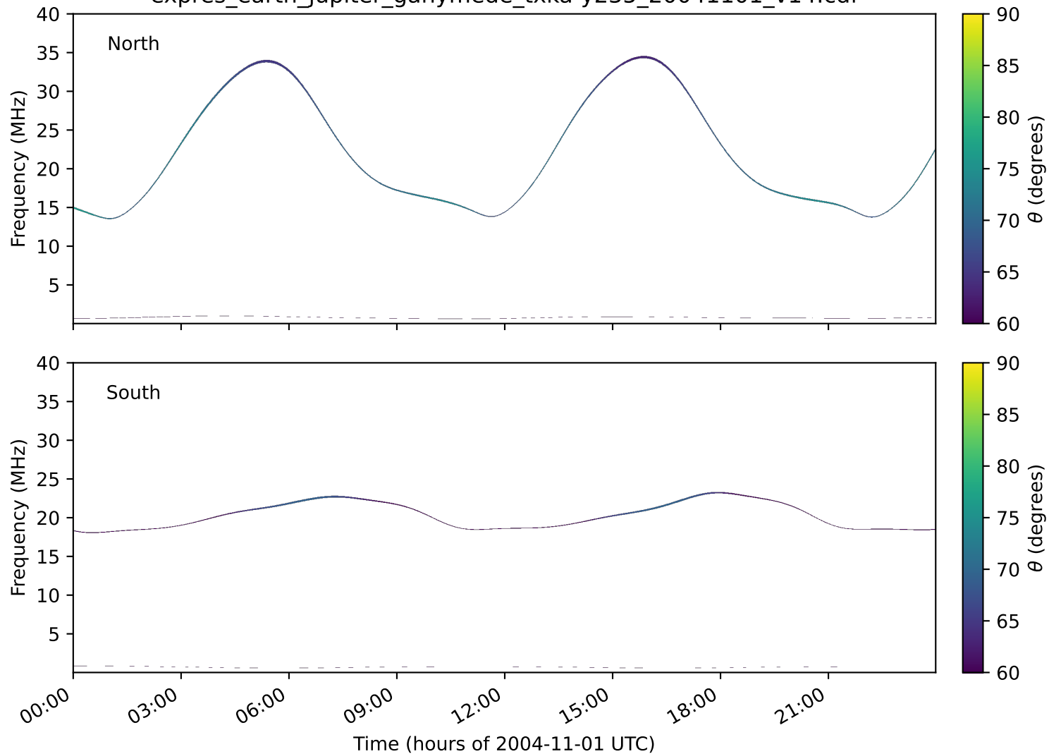
expres_earth_jupiter_ganymede_txka-y235_20041101_v14.cdf
