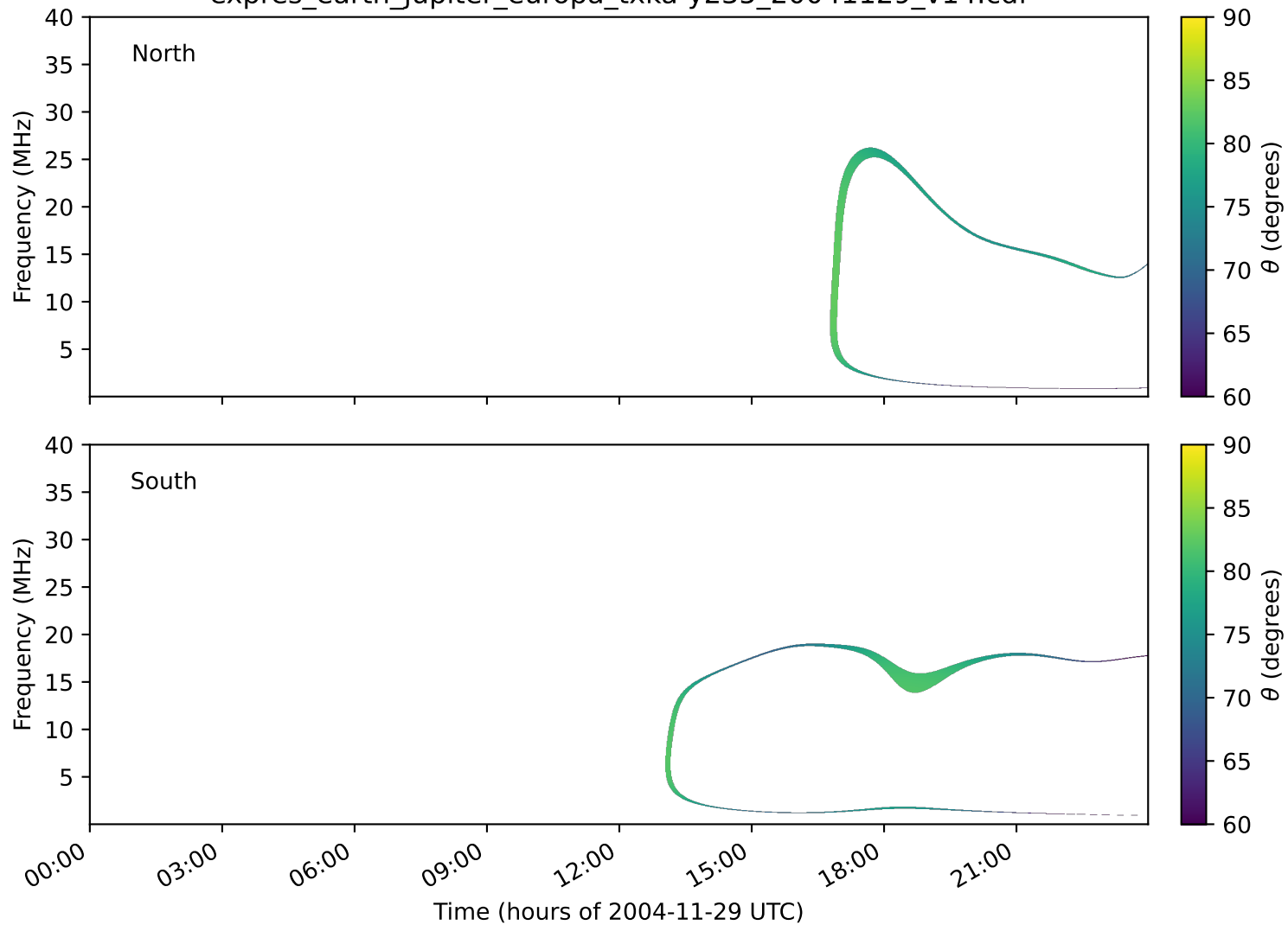
expres_earth_jupiter_europa_txka-y235_20041129_v14.cdf
