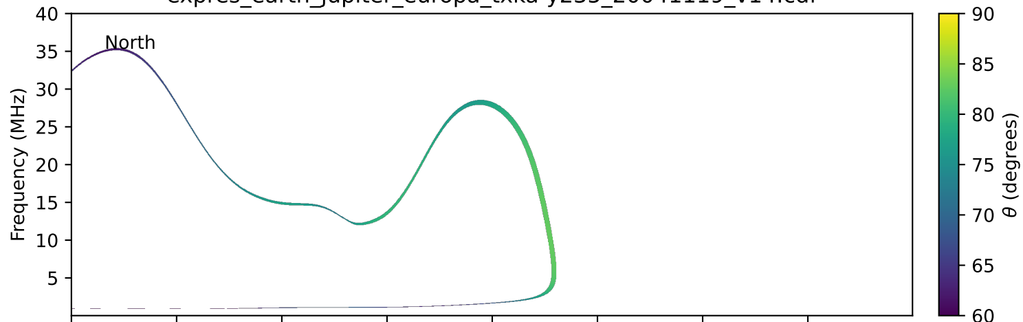
expres_earth_jupiter_europa_txka-y235_20041119_v14.cdf
