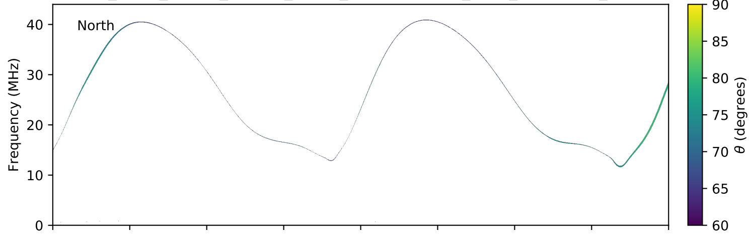
expres_earth_jupiter_europa_jrm09_lossc-wid1deg_3kev_20041130_v11.cdf
