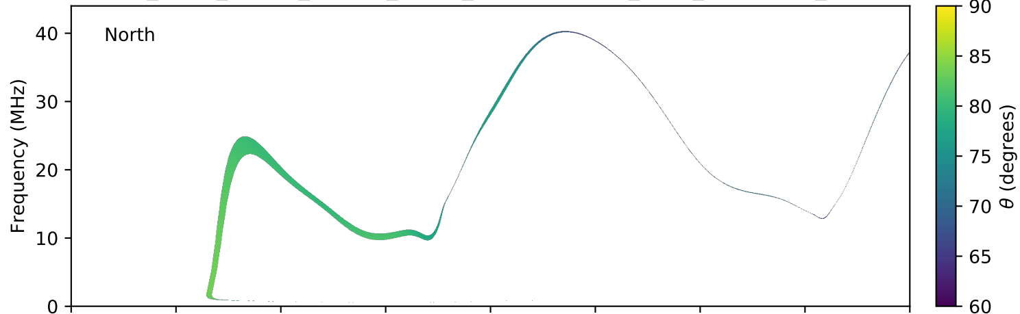
expres_earth_jupiter_europa_jrm09_lossc-wid1deg_3kev_20041125_v11.cdf
