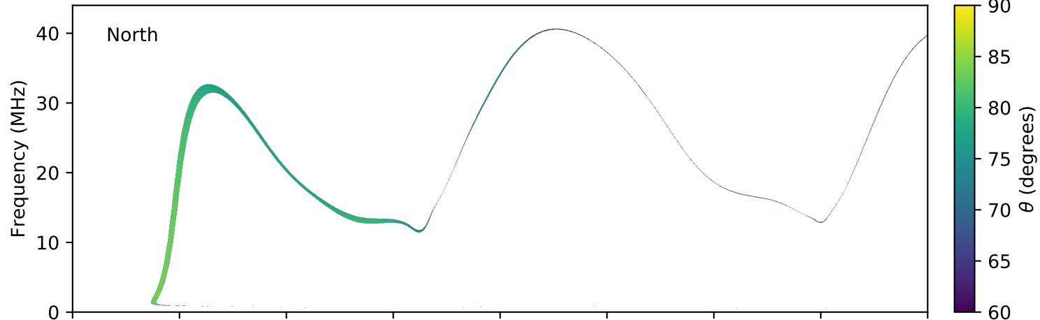
expres_earth_jupiter_europa_jrm09_lossc-wid1deg_3kev_20041118_v11.cdf
