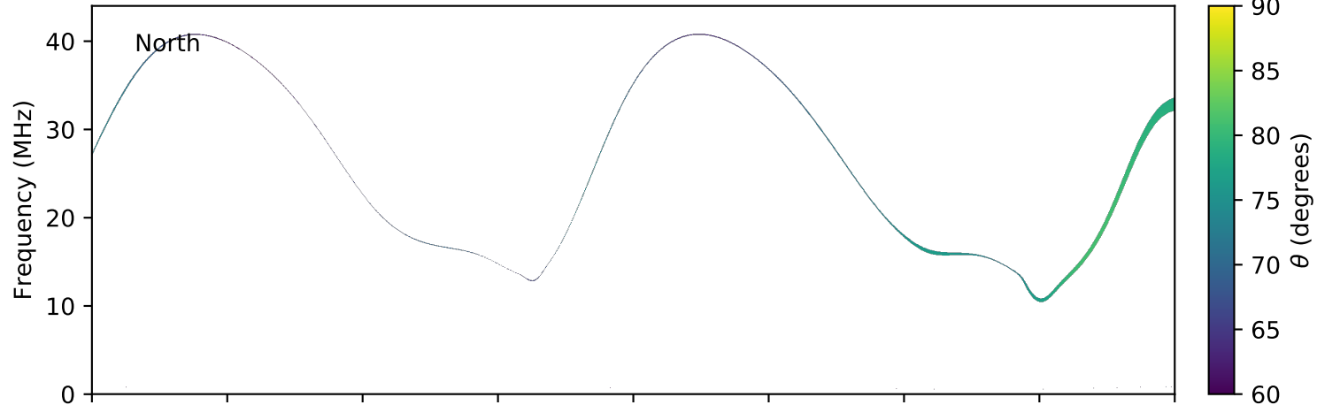
expres_earth_jupiter_europa_jrm09_lossc-wid1deg_3kev_20041104_v11.cdf
