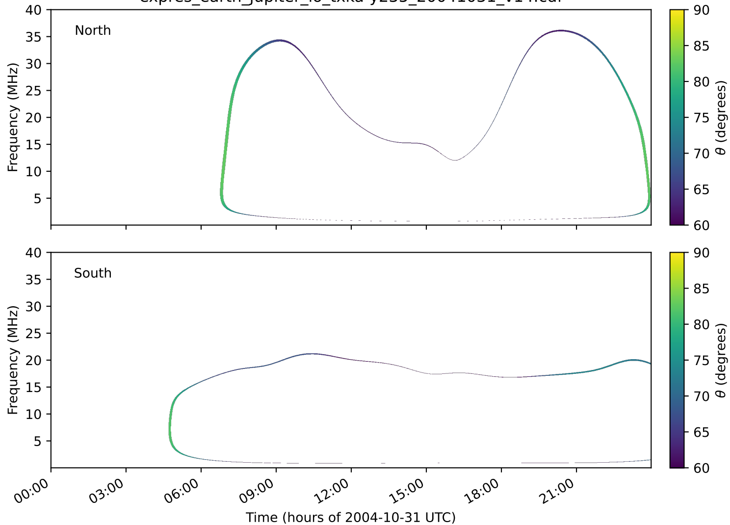
expres_earth_jupiter_io_txka-y235_20041031_v14.cdf
