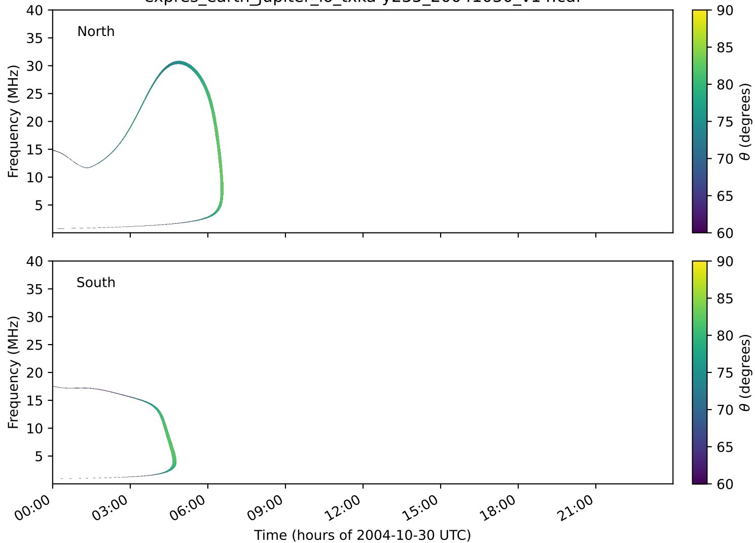
expres_earth_jupiter_io_txka-y235_20041030_v14.cdf
