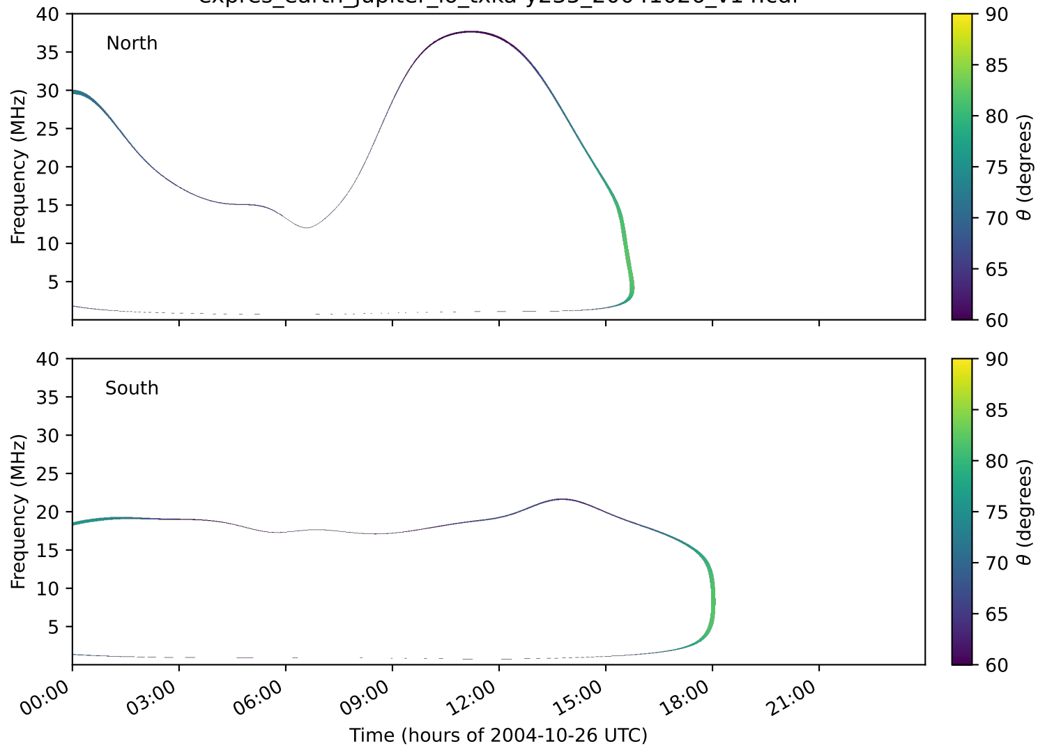
expres_earth_jupiter_io_txka-y235_20041026_v14.cdf
