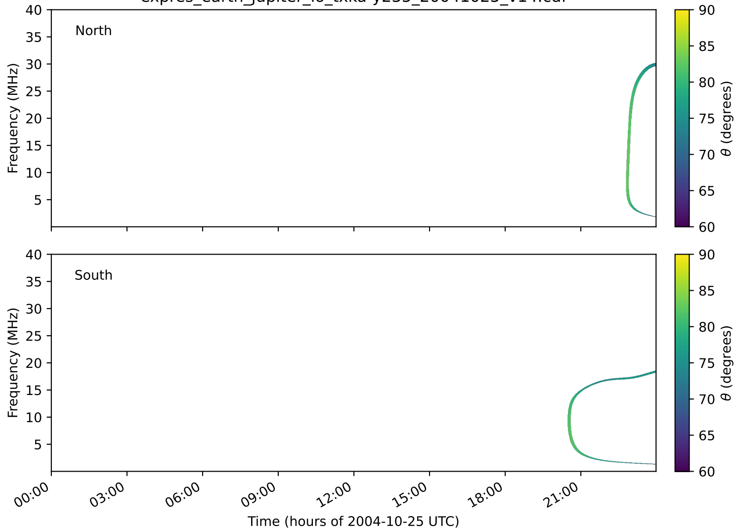
expres_earth_jupiter_io_txka-y235_20041025_v14.cdf
