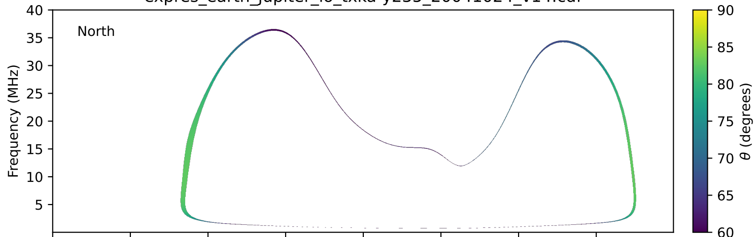
expres_earth_jupiter_io_txka-y235_20041024_v14.cdf
