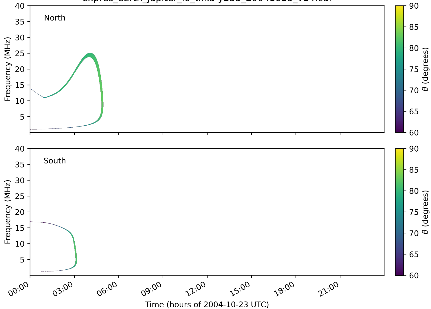
expres_earth_jupiter_io_txka-y235_20041023_v14.cdf
