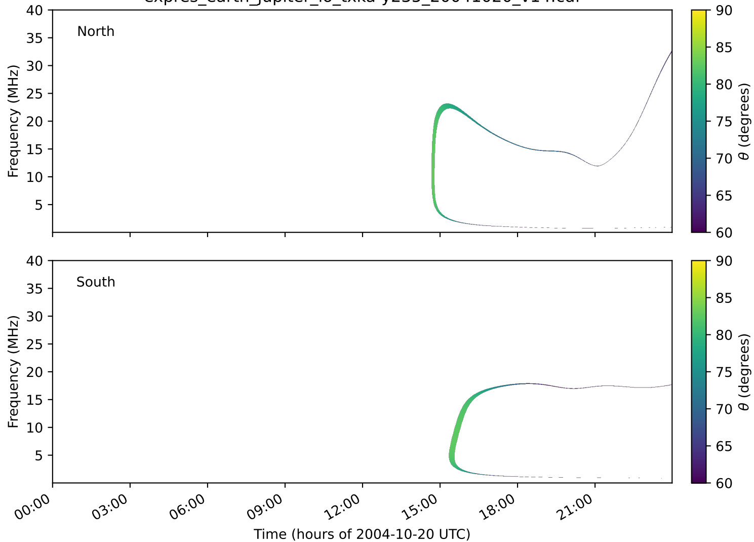
expres_earth_jupiter_io_txka-y235_20041020_v14.cdf
