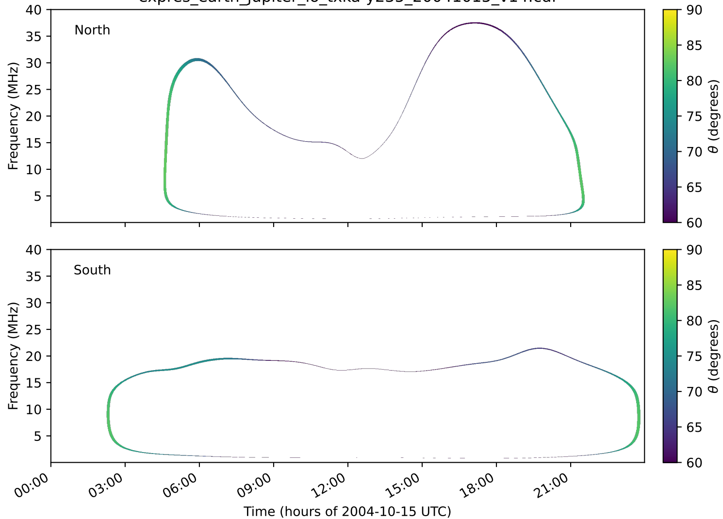
expres_earth_jupiter_io_txka-y235_20041015_v14.cdf
