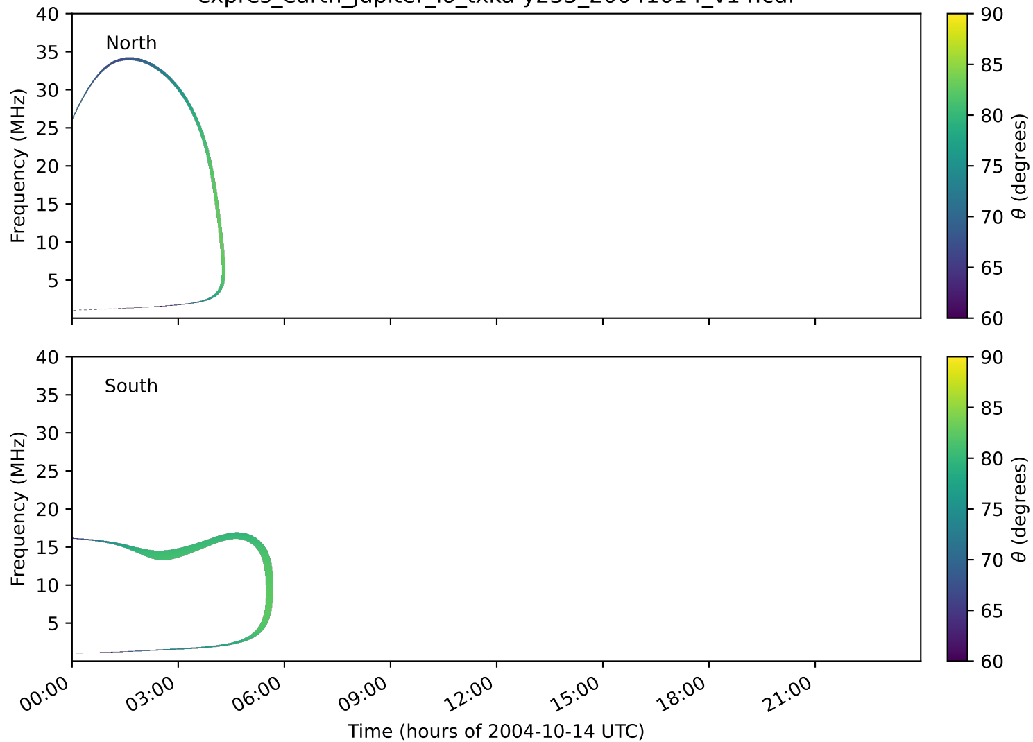
expres_earth_jupiter_io_txka-y235_20041014_v14.cdf
