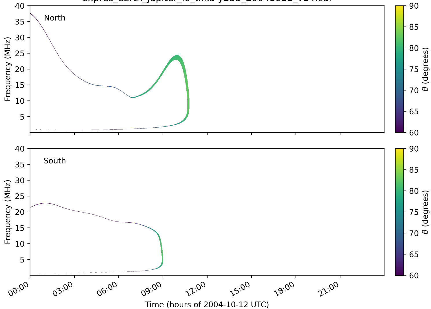
expres_earth_jupiter_io_txka-y235_20041012_v14.cdf
