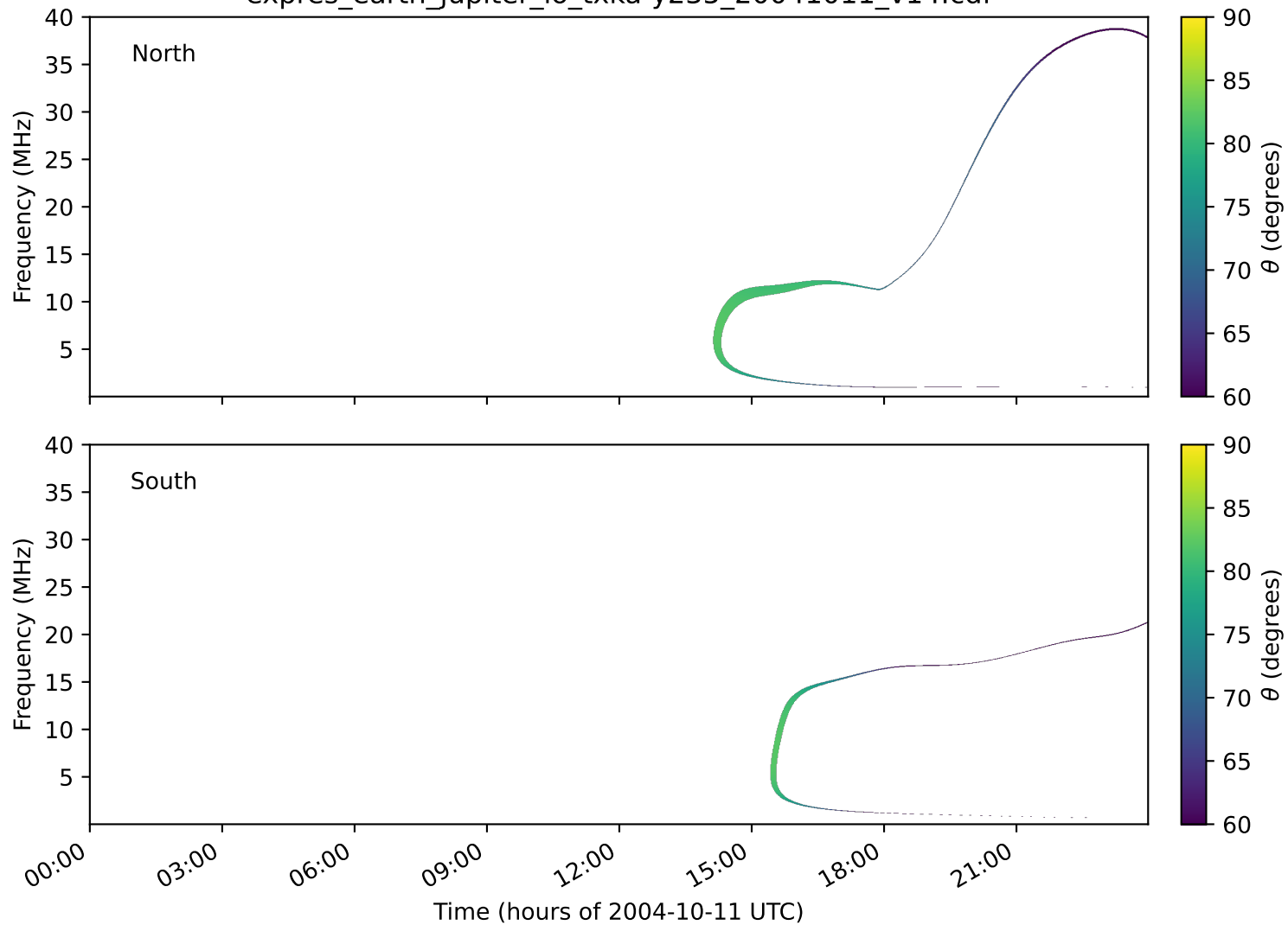
expres_earth_jupiter_io_txka-y235_20041011_v14.cdf
