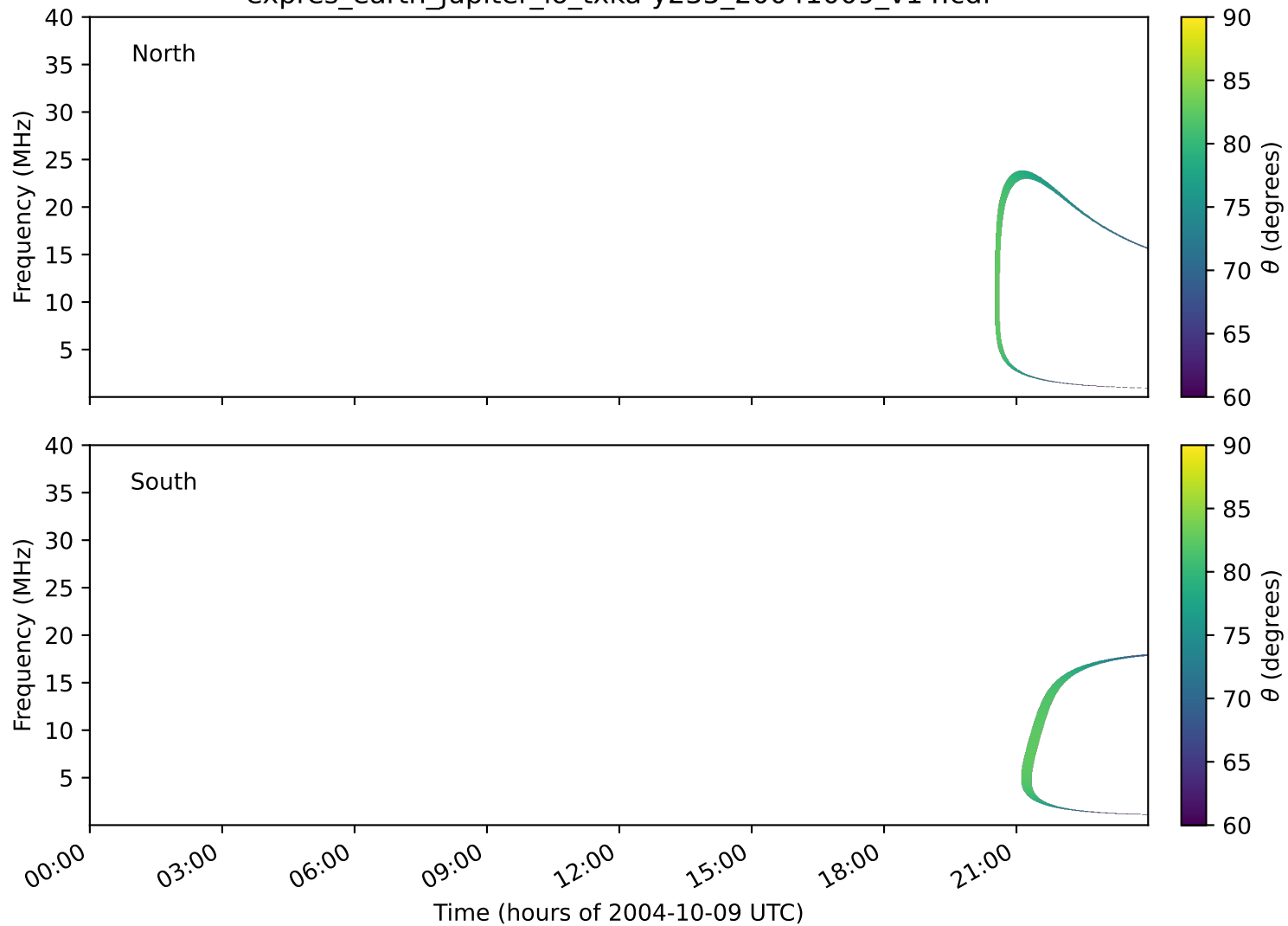
expres_earth_jupiter_io_txka-y235_20041009_v14.cdf
