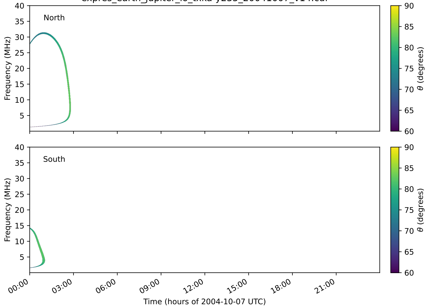
expres_earth_jupiter_io_txka-y235_20041007_v14.cdf
