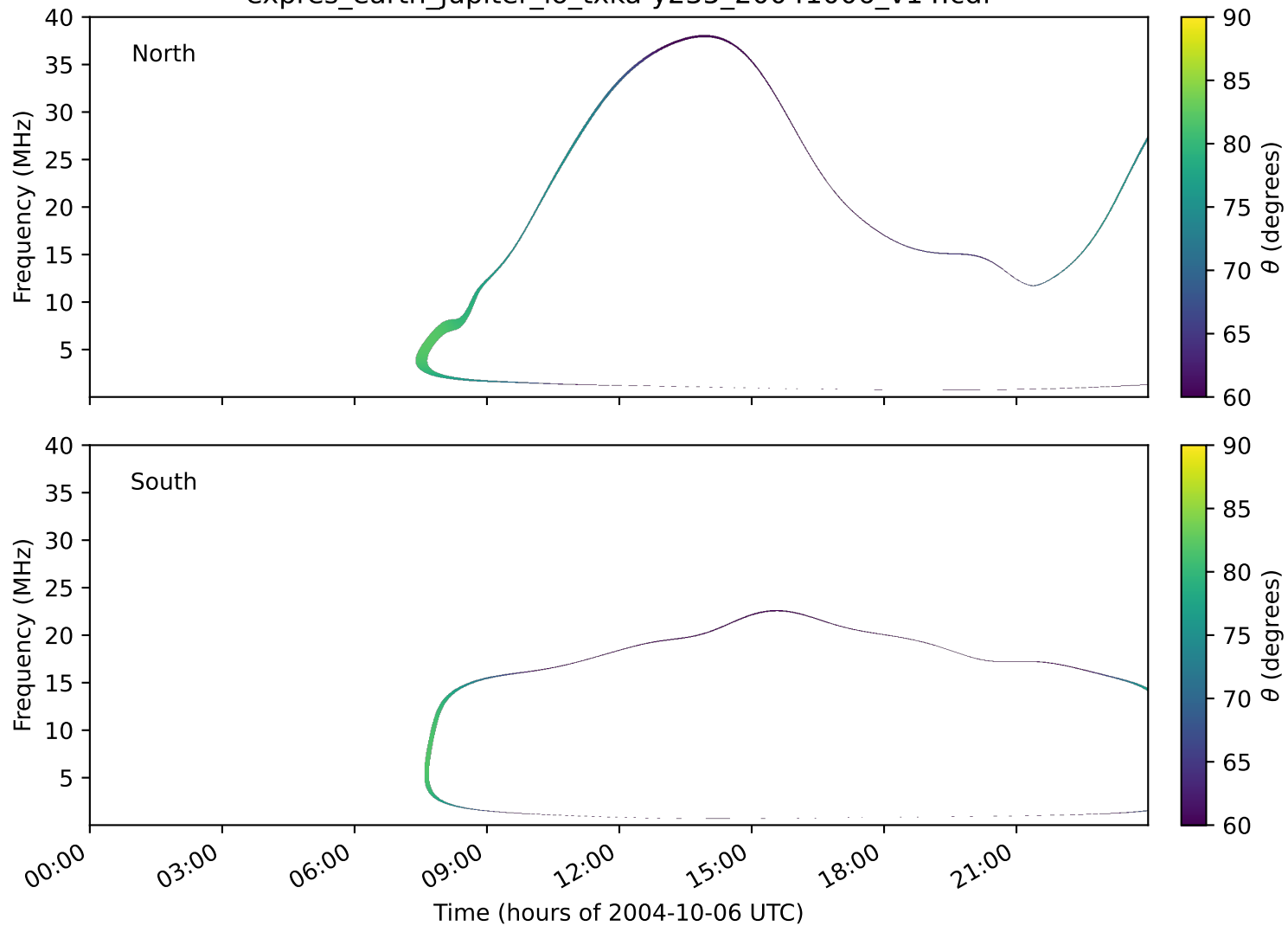
expres_earth_jupiter_io_txka-y235_20041006_v14.cdf
