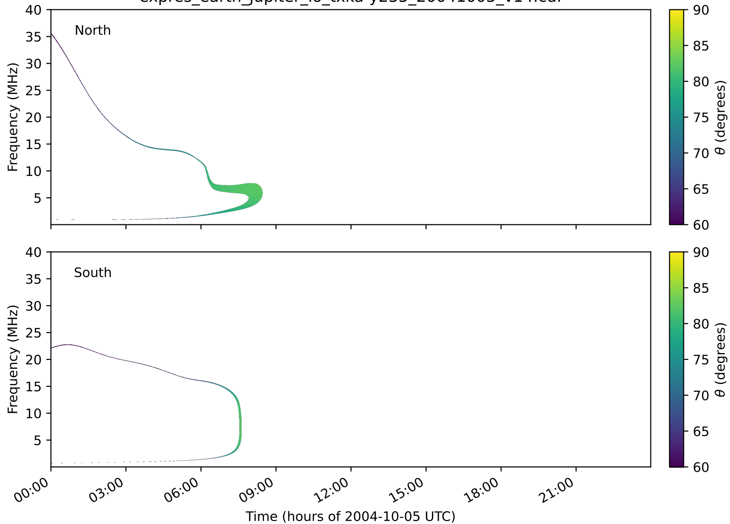
expres_earth_jupiter_io_txka-y235_20041005_v14.cdf
