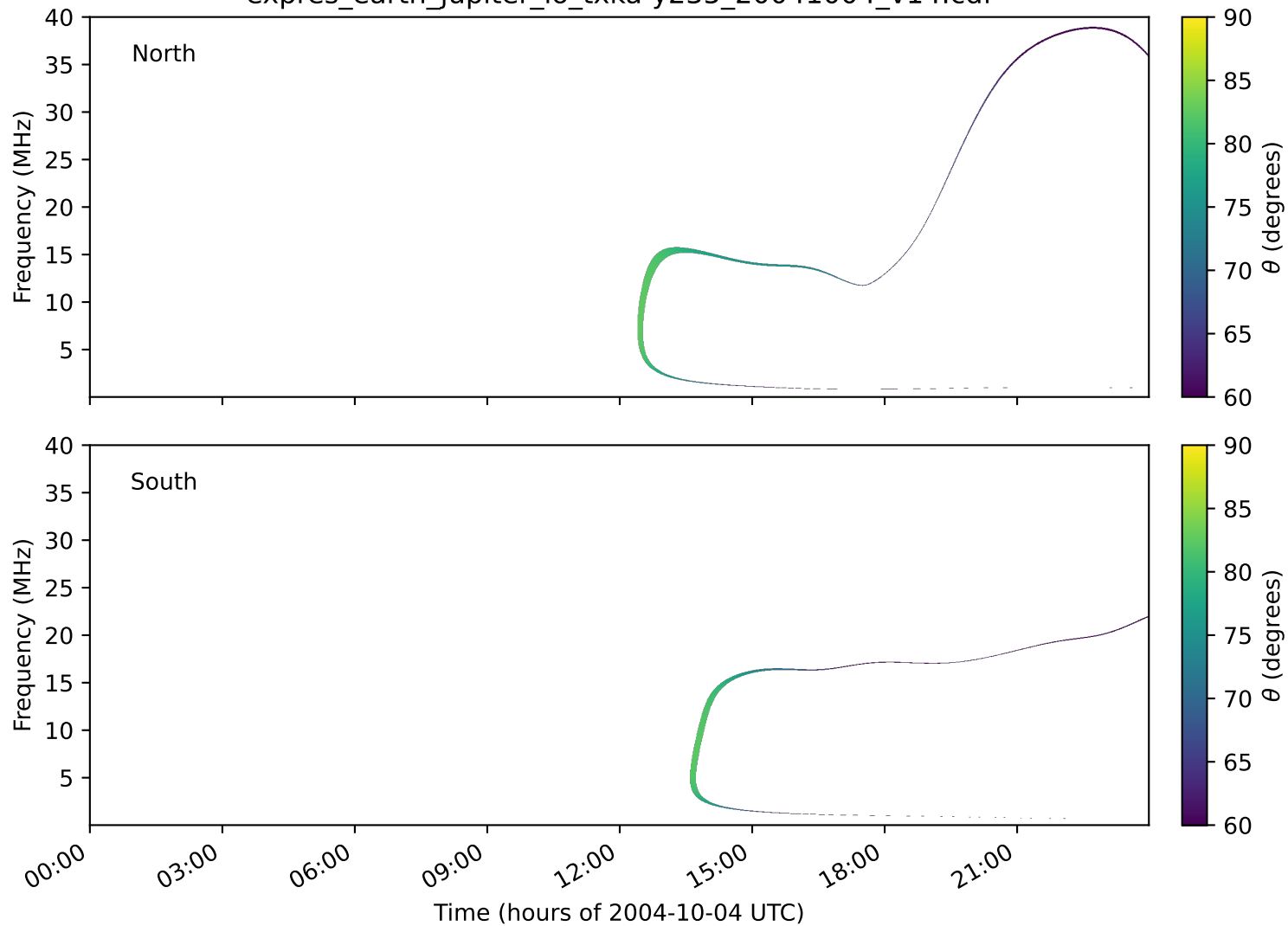
expres_earth_jupiter_io_txka-y235_20041004_v14.cdf
