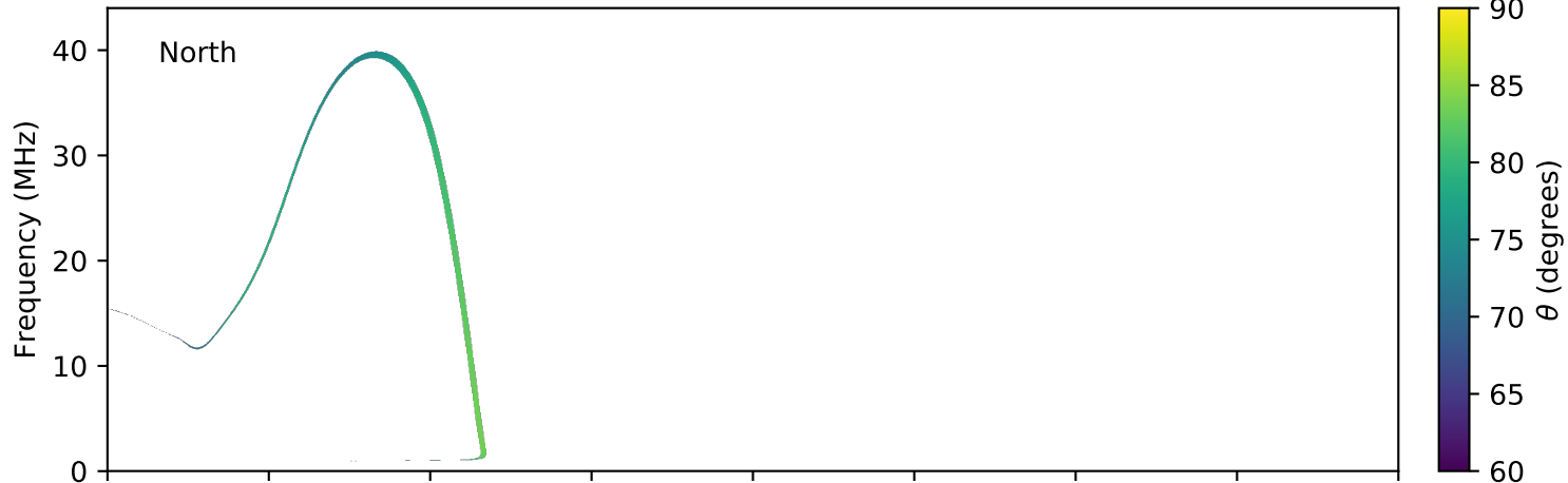
expres_earth_jupiter_io_jrm09_lossc-wid1deg_3kev_20041030_v11.cdf
