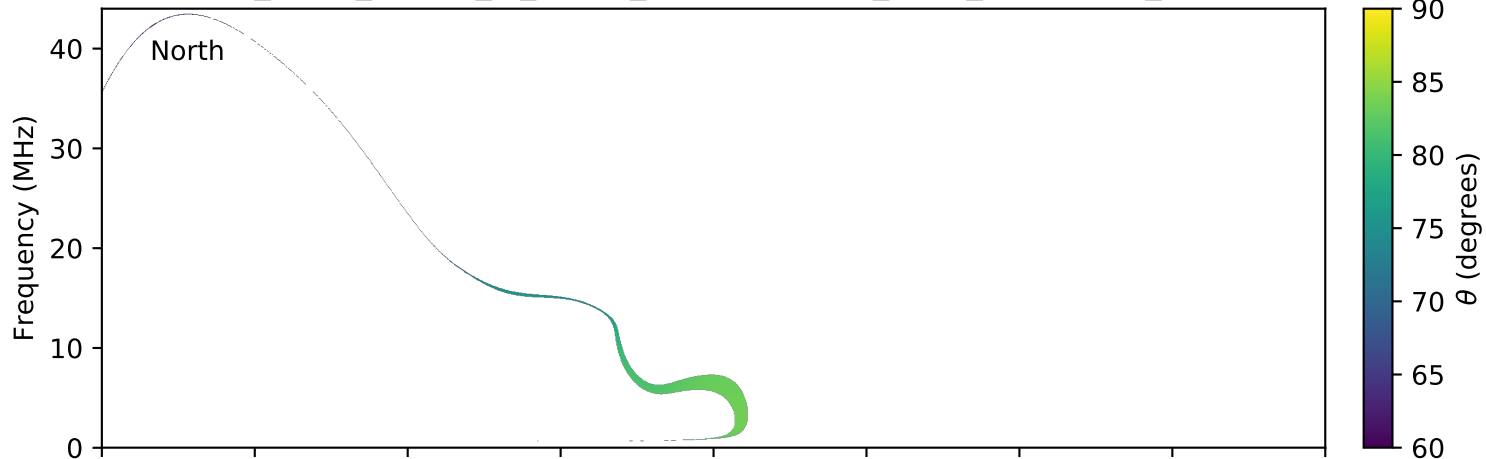
expres_earth_jupiter_io_jrm09_lossc-wid1deg_3kev_20041028_v11.cdf
