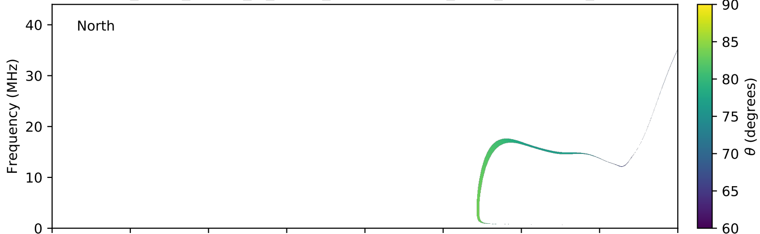
expres_earth_jupiter_io_jrm09_lossc-wid1deg_3kev_20041027_v11.cdf
