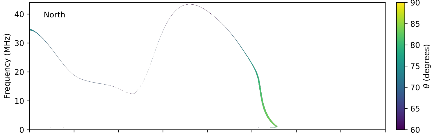
expres_earth_jupiter_io_jrm09_lossc-wid1deg_3kev_20041026_v11.cdf
