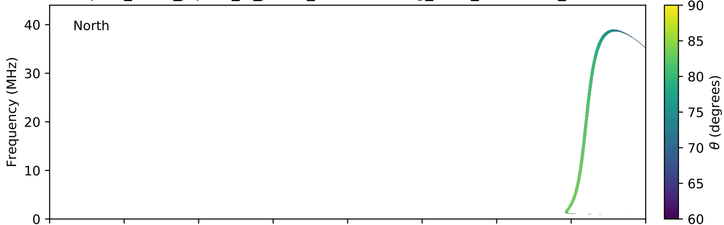
expres_earth_jupiter_io_jrm09_lossc-wid1deg_3kev_20041018_v11.cdf
