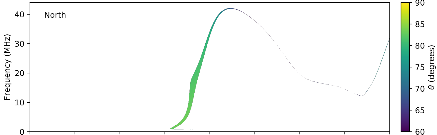
expres_earth_jupiter_io_jrm09_lossc-wid1deg_3kev_20041013_v11.cdf
