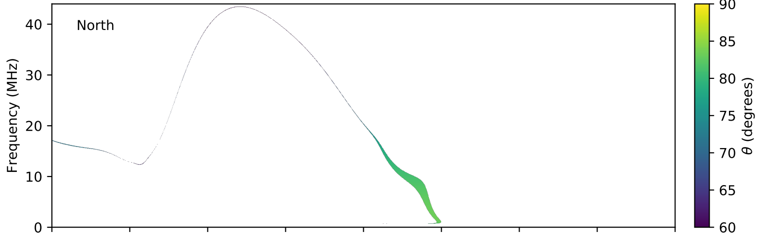
expres_earth_jupiter_io_jrm09_lossc-wid1deg_3kev_20041010_v11.cdf
