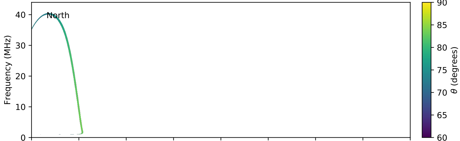
expres_earth_jupiter_io_jrm09_lossc-wid1deg_3kev_20041007_v11.cdf
