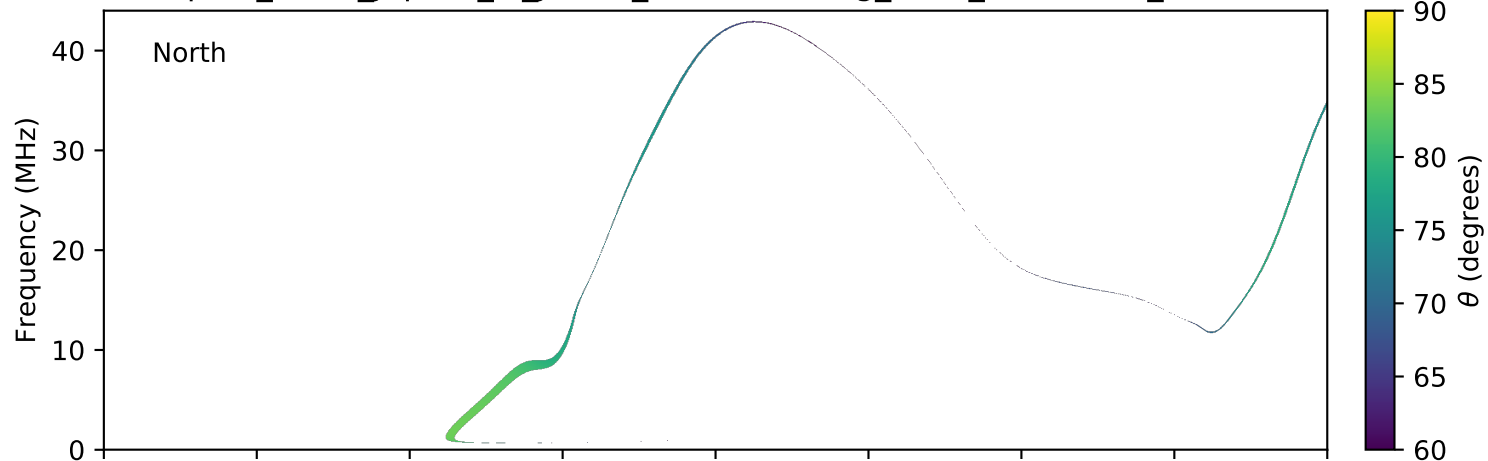
expres_earth_jupiter_io_jrm09_lossc-wid1deg_3kev_20041006_v11.cdf
