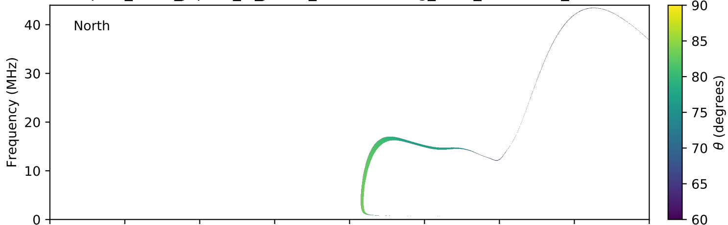
expres_earth_jupiter_io_jrm09_lossc-wid1deg_3kev_20041004_v11.cdf
