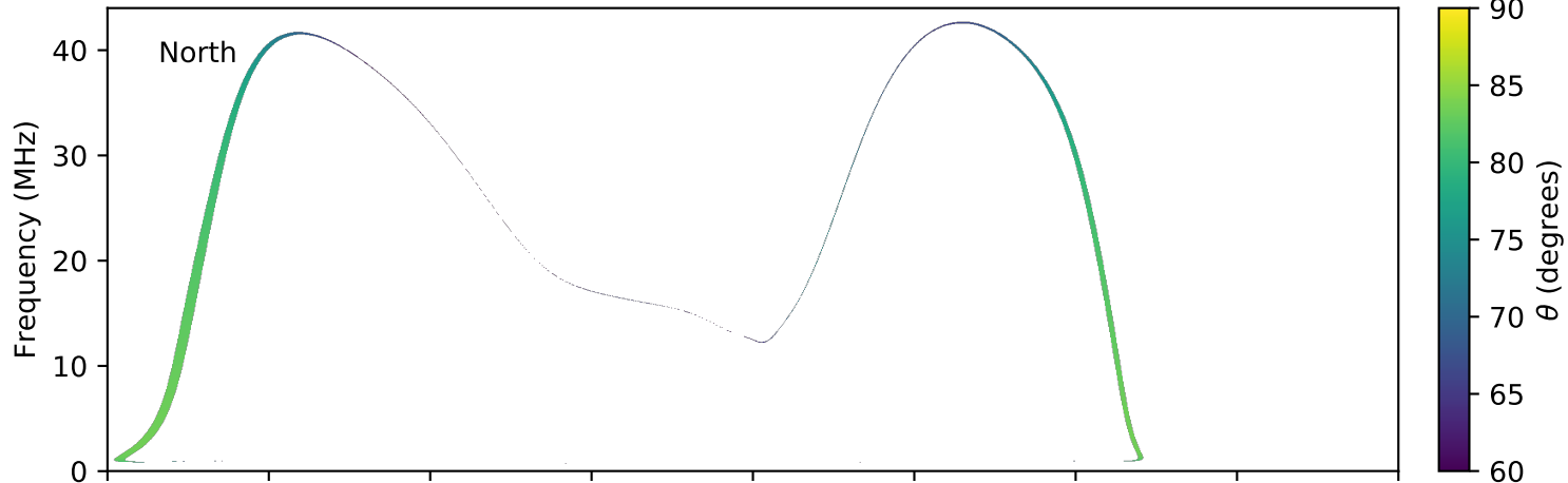
expres_earth_jupiter_io_jrm09_lossc-wid1deg_3kev_20041001_v11.cdf
