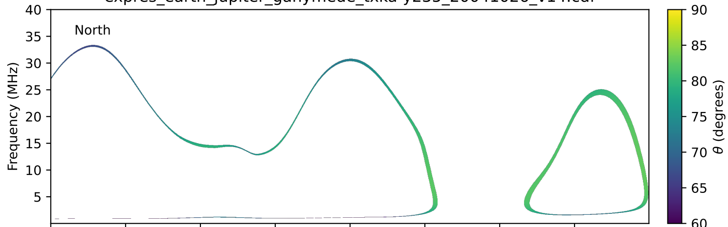
expres_earth_jupiter_ganymede_txka-y235_20041026_v14.cdf
