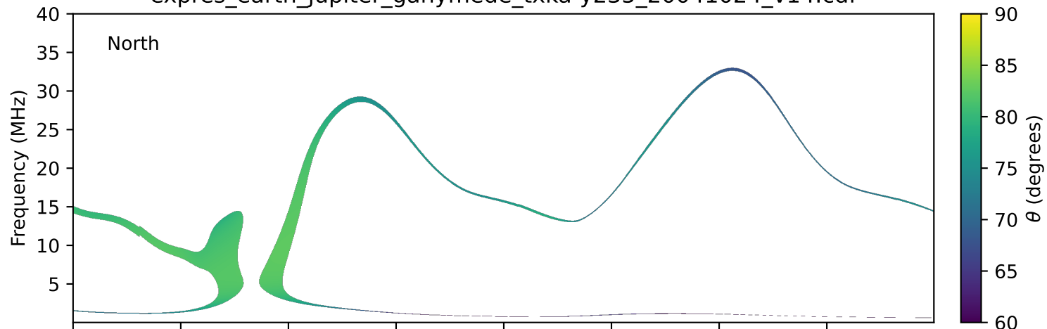
expres_earth_jupiter_ganymede_txka-y235_20041024_v14.cdf
