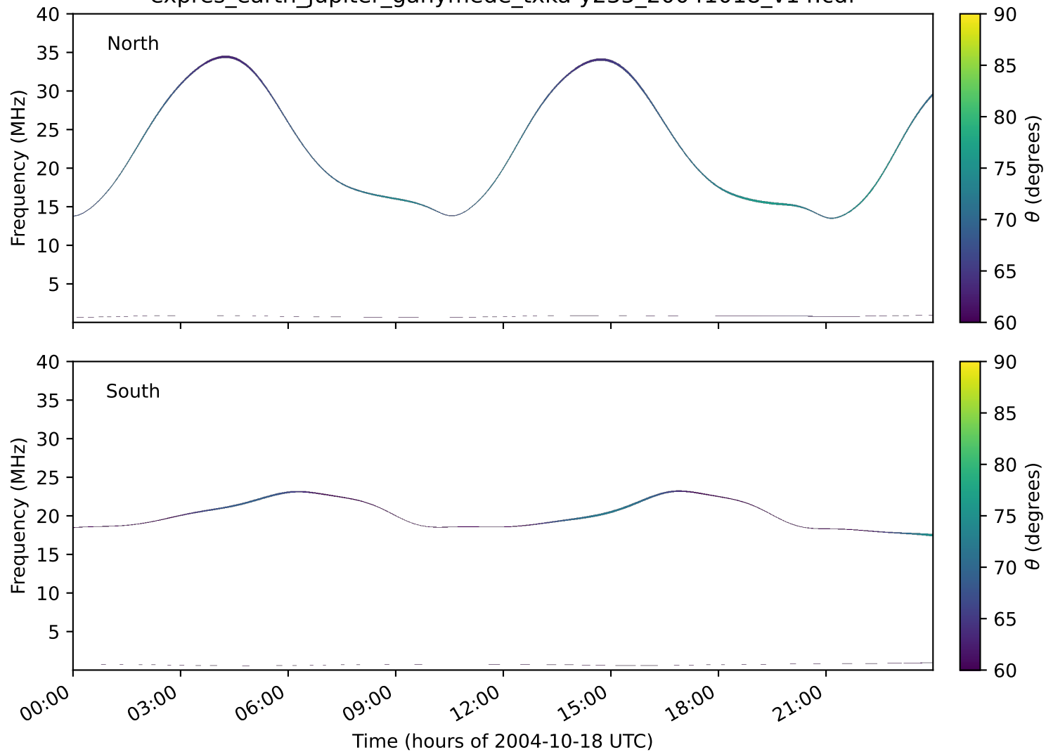
expres_earth_jupiter_ganymede_txka-y235_20041018_v14.cdf
