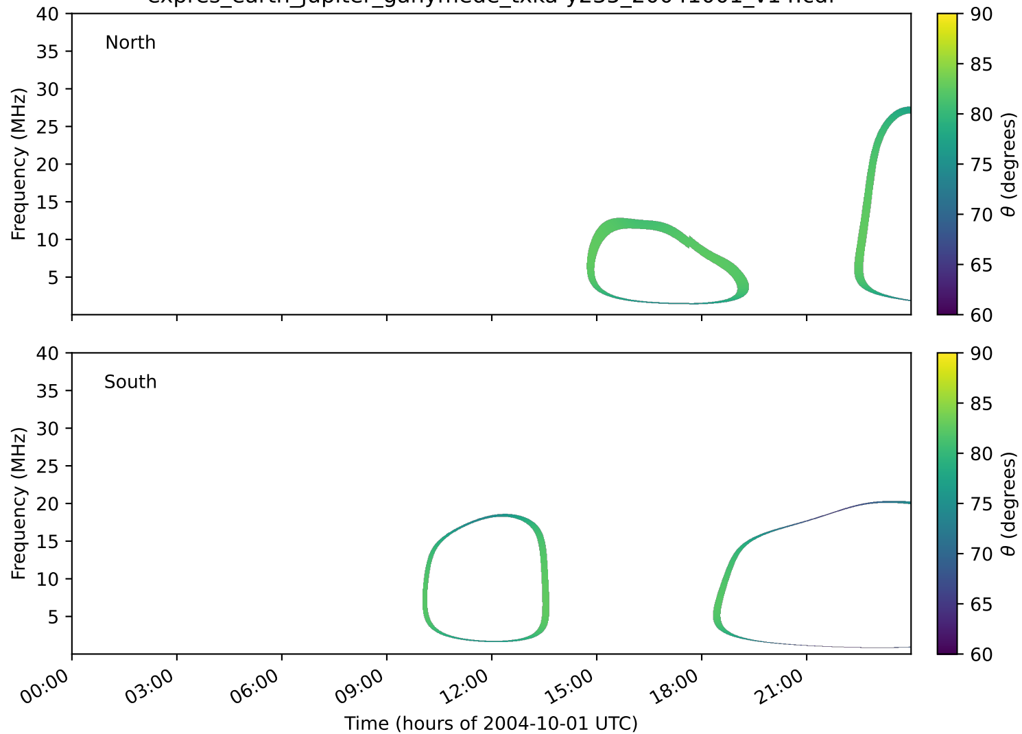
expres_earth_jupiter_ganymede_txka-y235_20041001_v14.cdf
